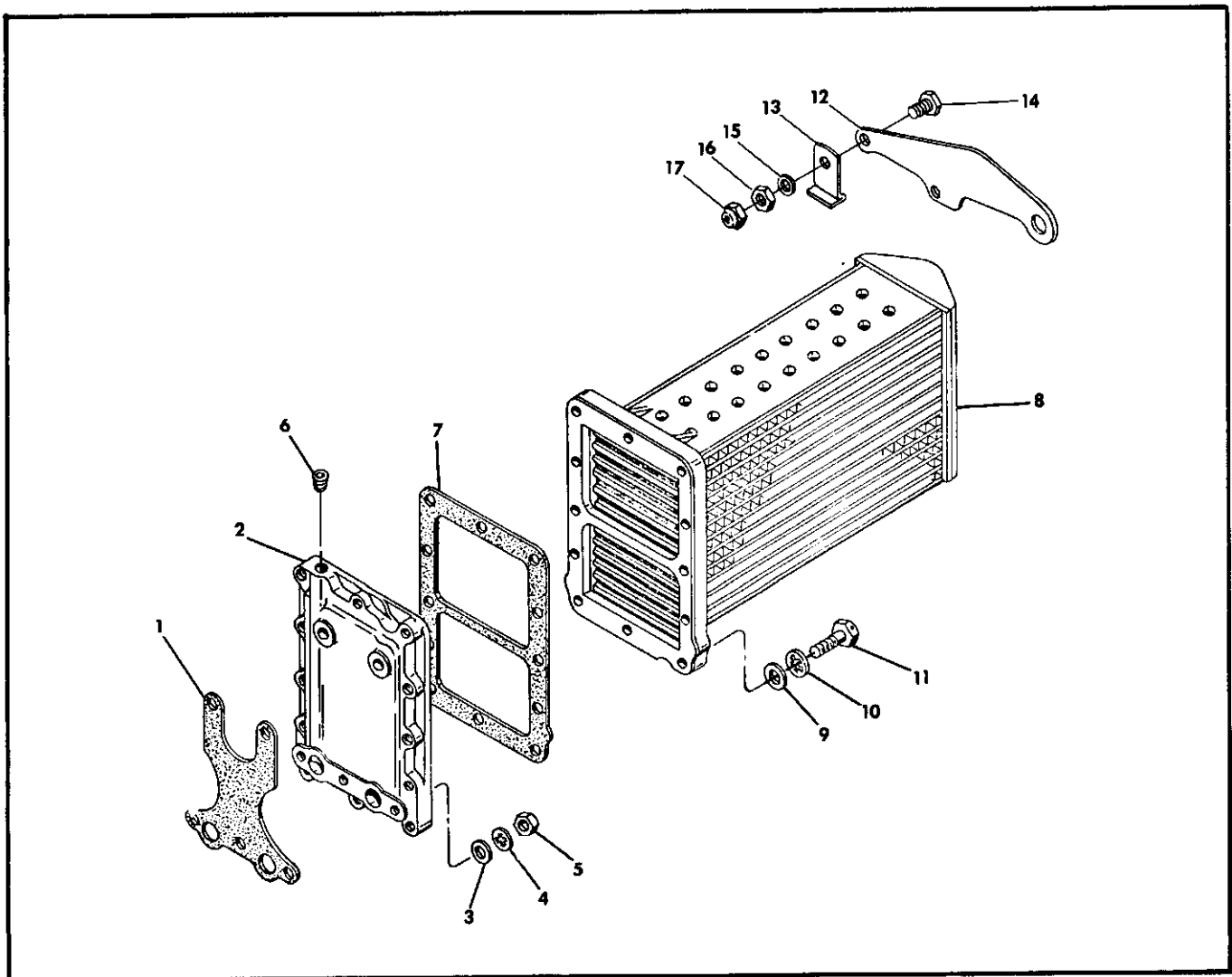
Figure 22. Oil Cooler.
