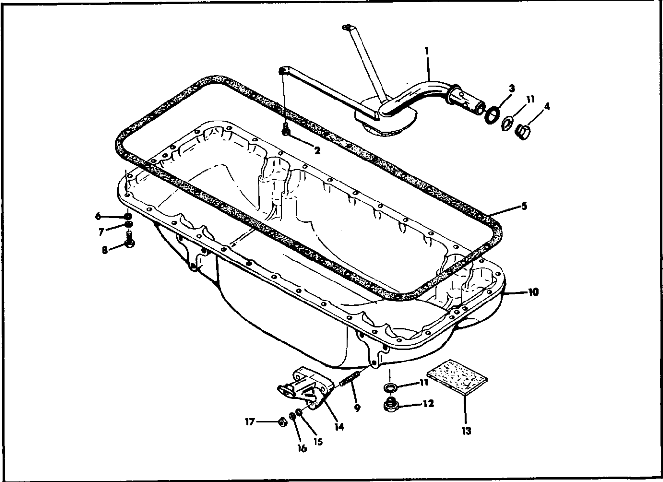
Figure 25. Oil Sump.
