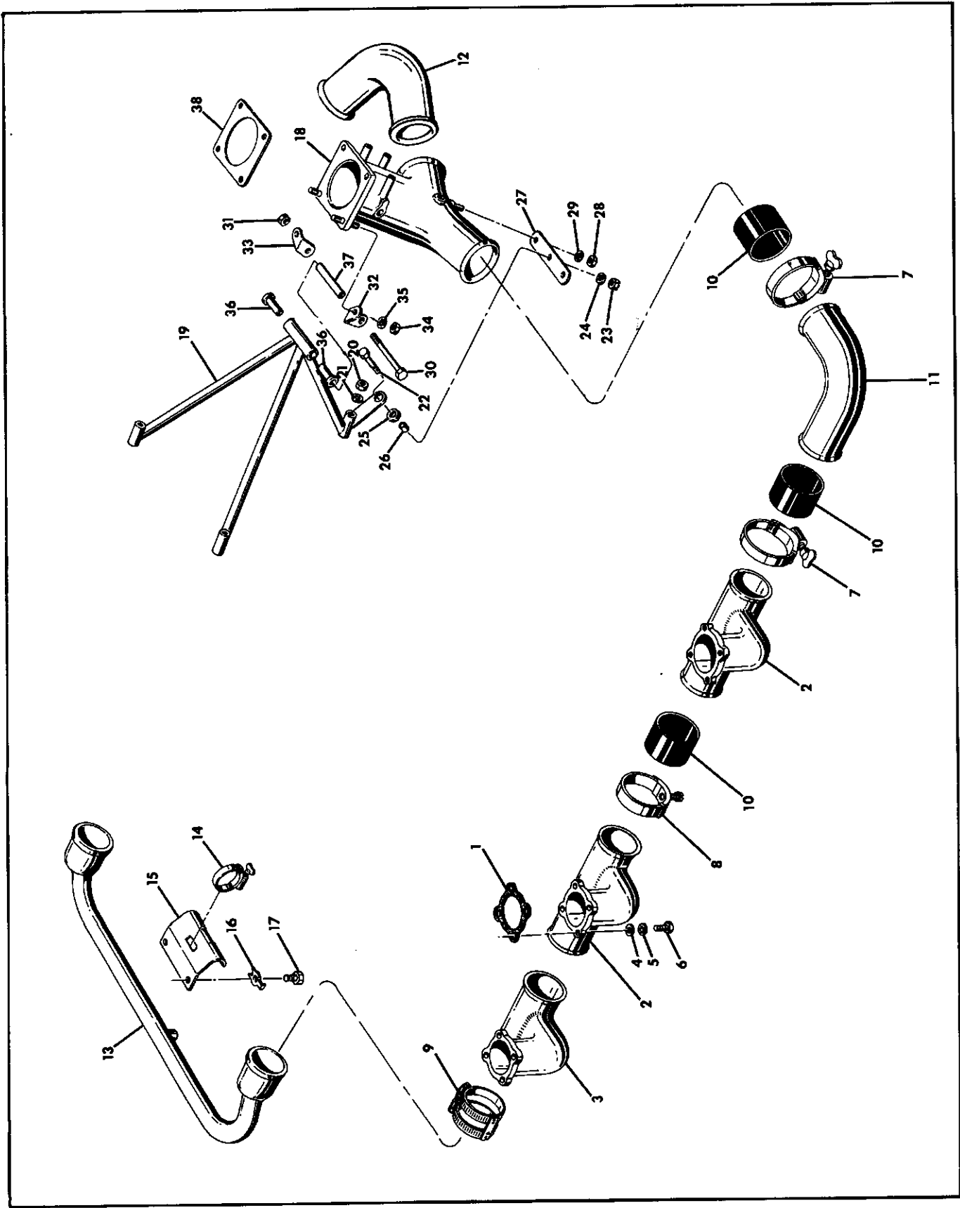
Figure 29. Induction System.
