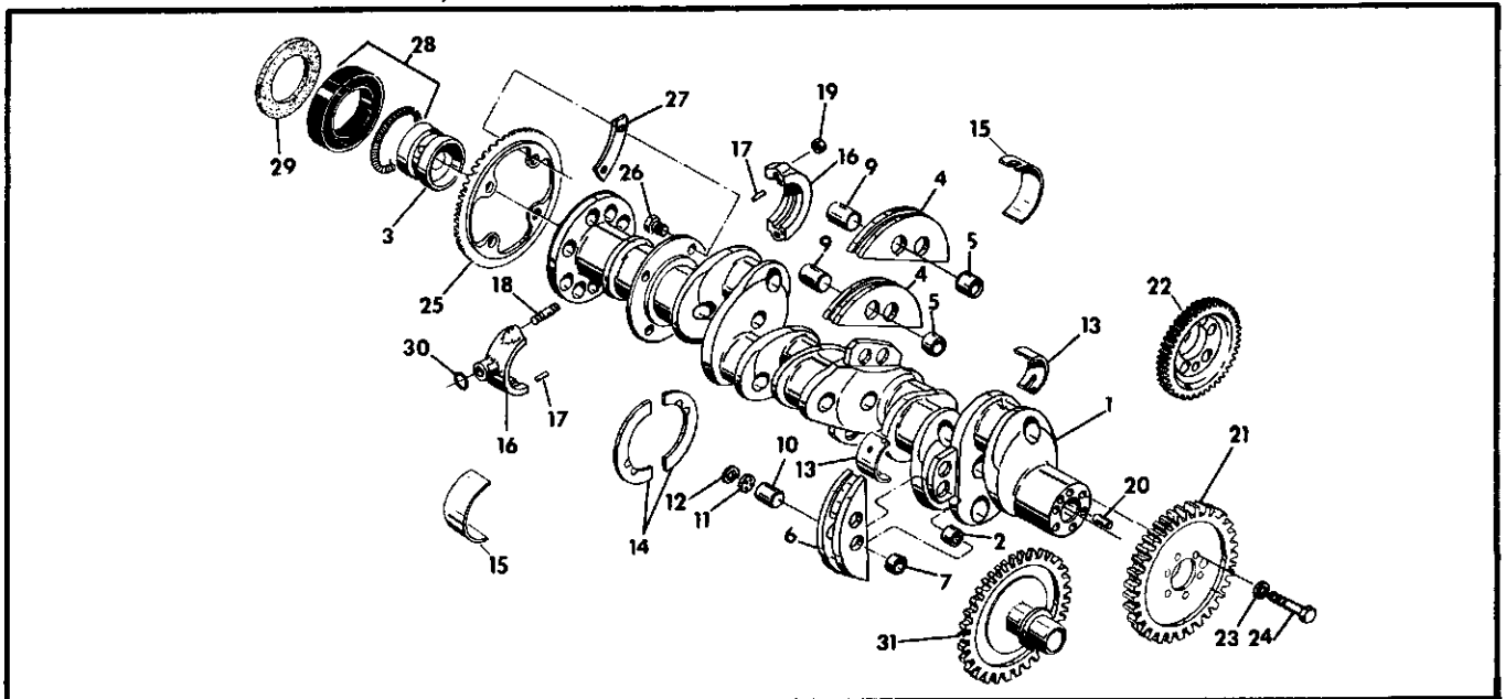
Figure 8. Crankshaft Group.
