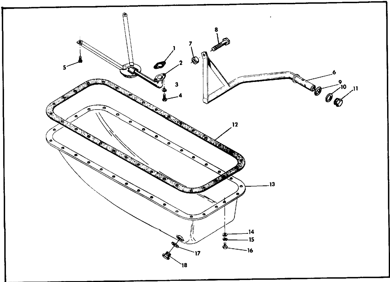
Figure 24. Oil Sump.
