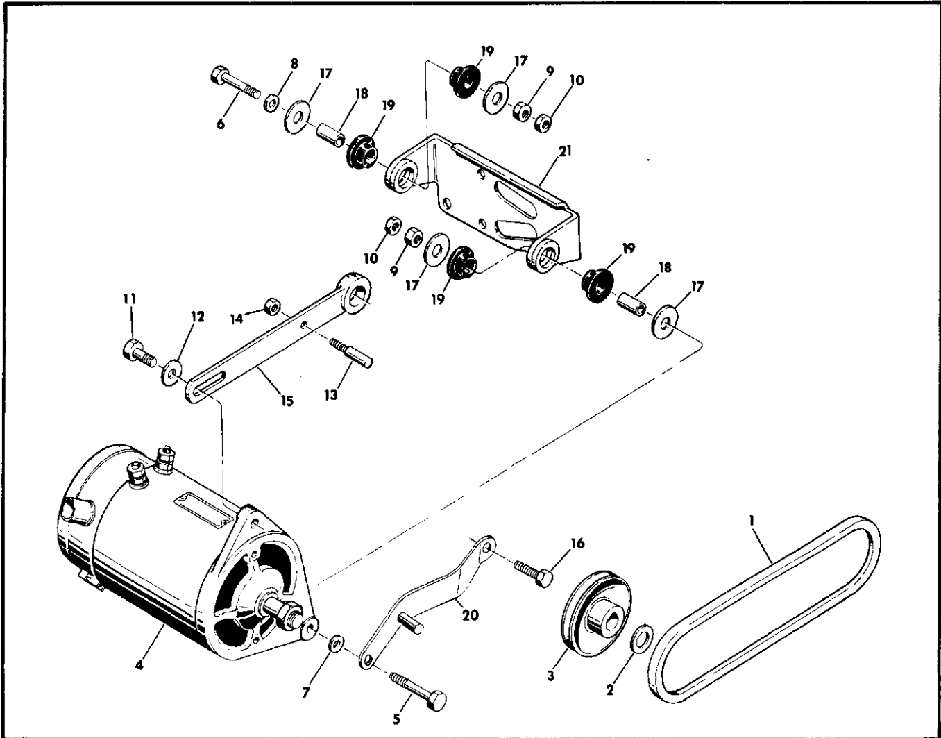
Figure 20. Generator Assembly.
