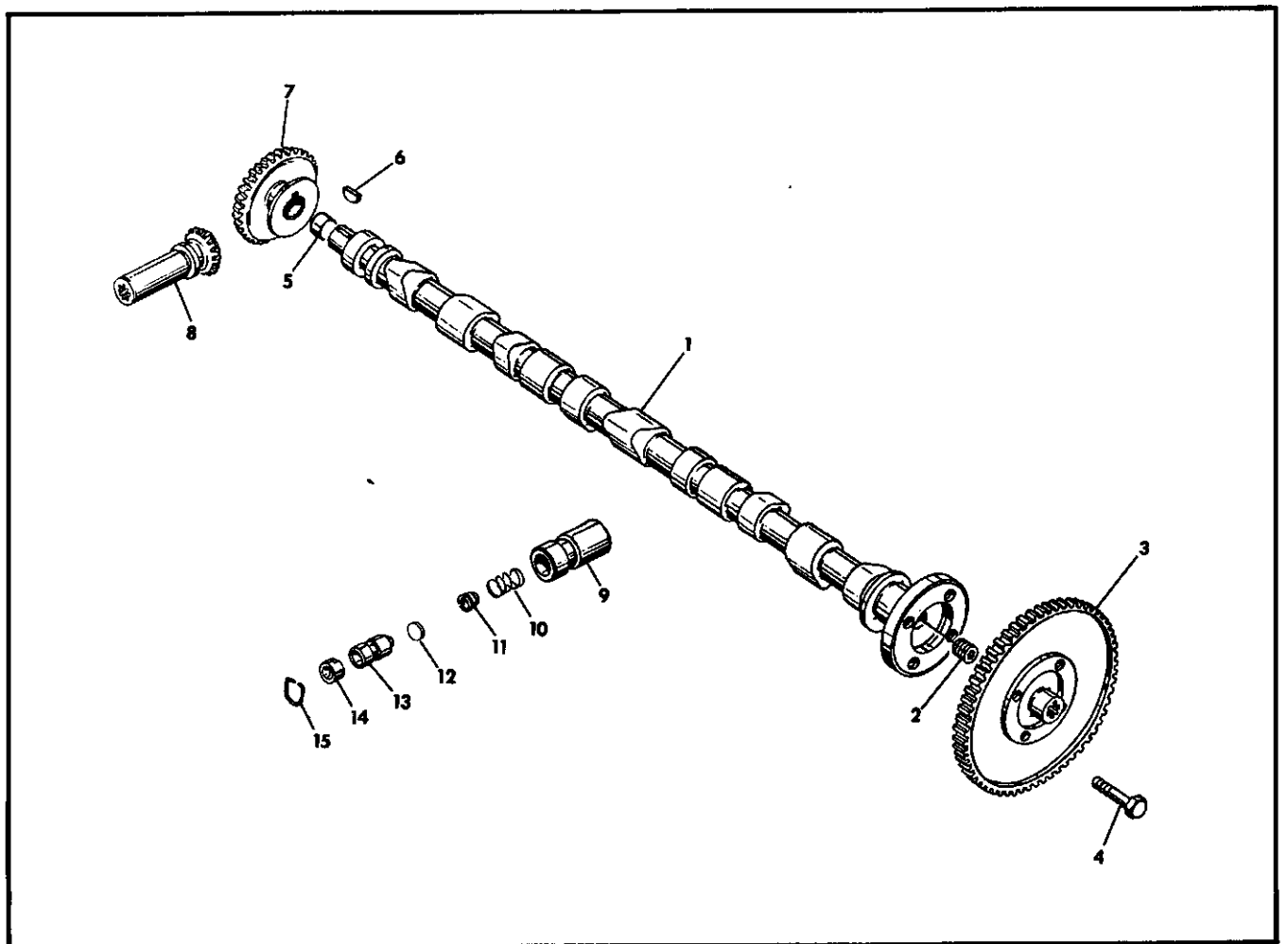
Figure 10. Camshaft Group.
