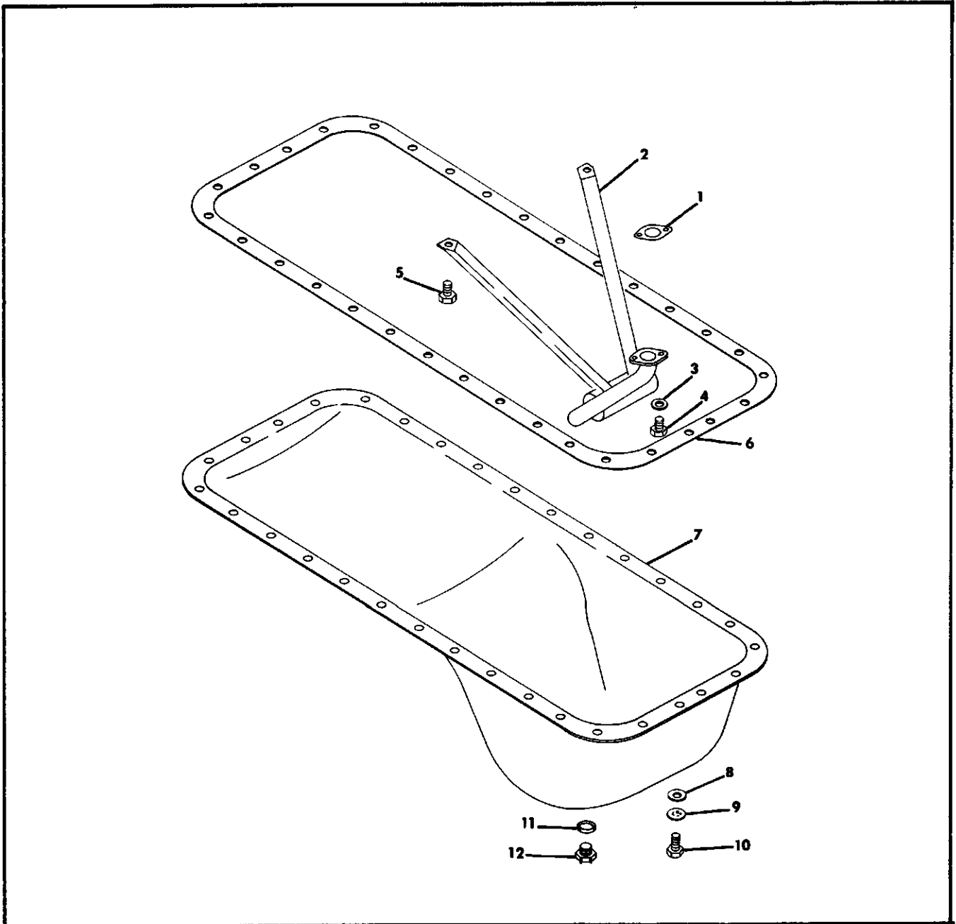
Figure 26. Oil Sump
