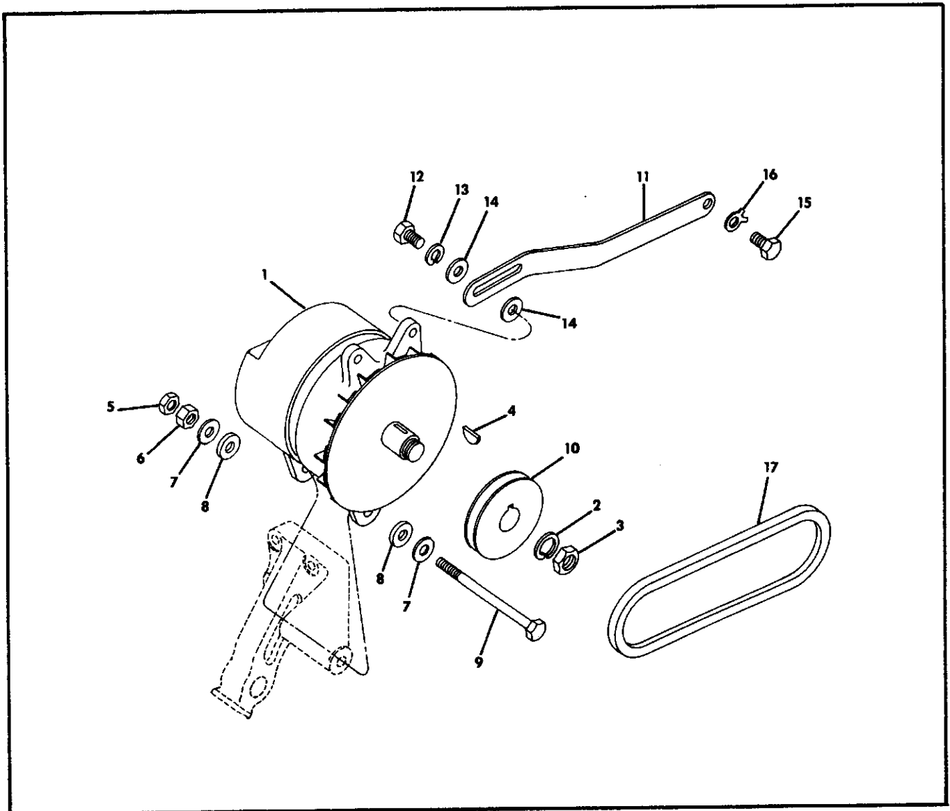
Figure 21. Alternator Assembly
