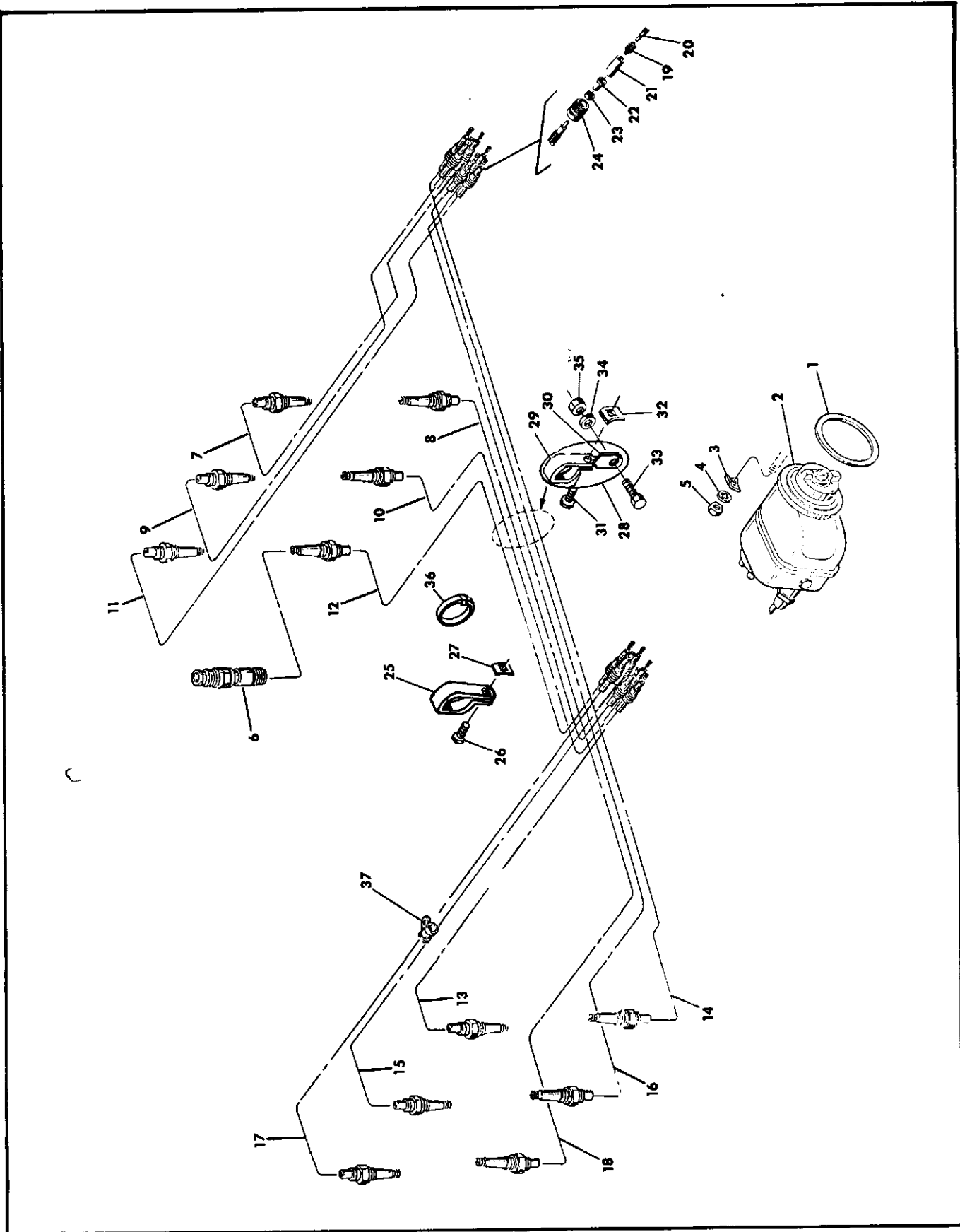
Figure 35. Ignition System.
